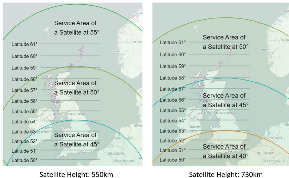
Figure 1 Satellite Service Area from orbits relevant to the UK achieved from various inclinations. A satellite with a service beamwidth of 116°, placed at an inclination of 50° or higher can provide good visibility and coverage in the UK, including the northern parts. The service area is dependent on orbit height as well. Instantaneous service area of satellites changes dynamically with respect to their relative position - the presented plots show the service area limits for the specified inclination angles and heights over the UK.
